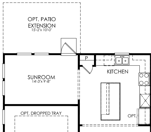
Sunroom Adds 147 SF
