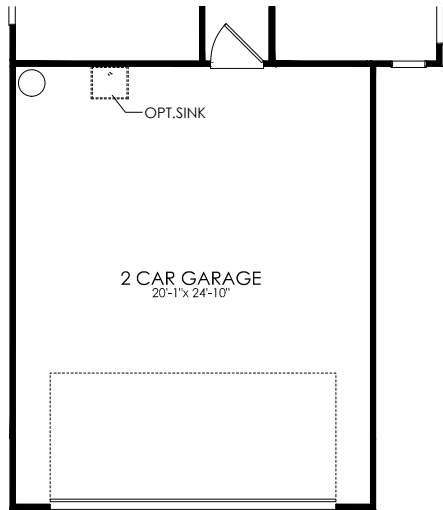
4' Garage Extension
